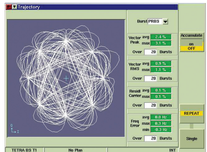
Figure 19. Trajectory Tile Maximized
