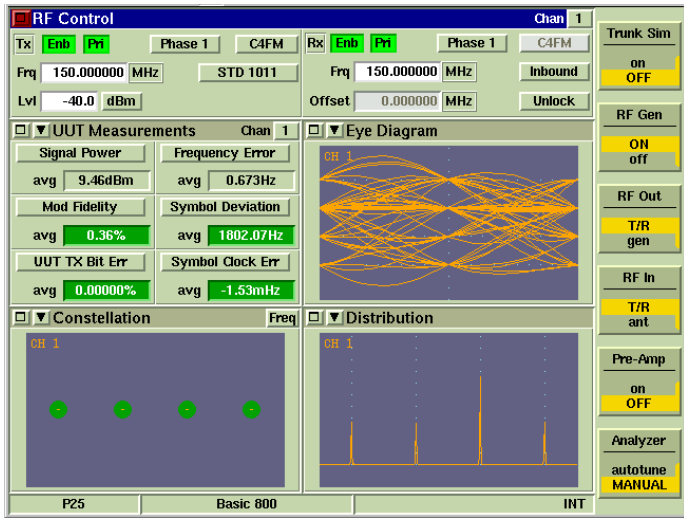
Figure 10. P25 Conventional
