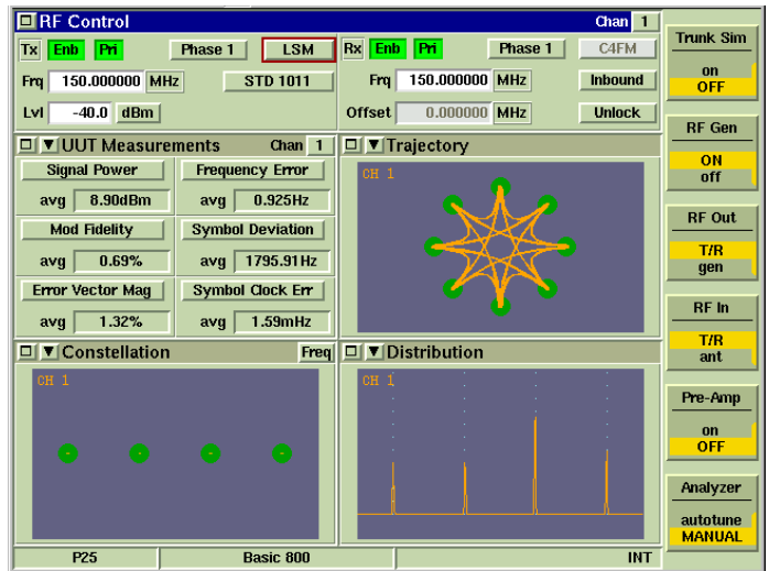
Figure 12. LSM Signal Analysis Screen
