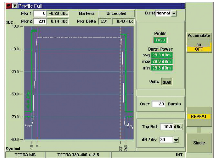
Figure 18. Profile Full Tile Maximized TETRA
