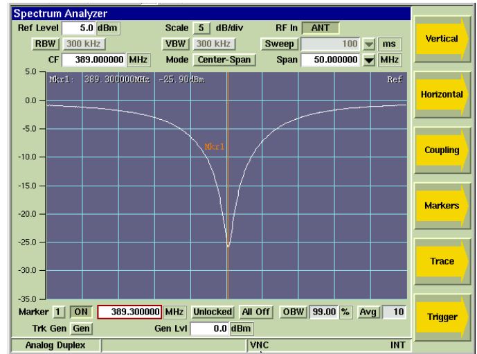
Figure 8. Spectrum Analyzer with Tracking Generator
