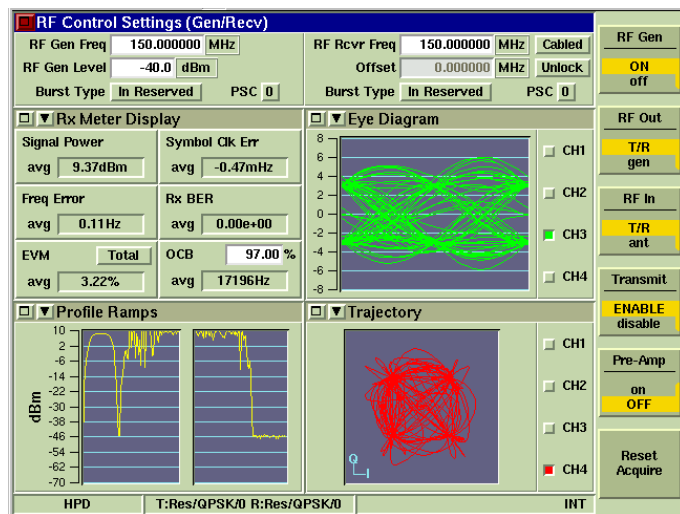
Figure 14. Example of HPD Tiles
