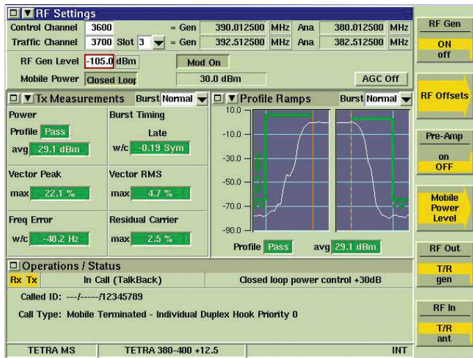
Figure 17. Example of TETRA MS Tiles
