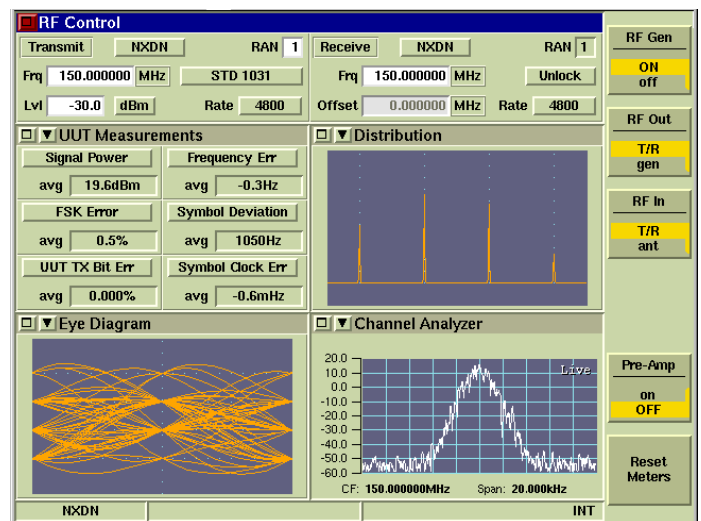
Figure 16. Example of NXDN Tiles
