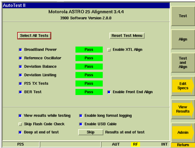
Figure 3. Motorola ASTRO 25 Radio Alignment
