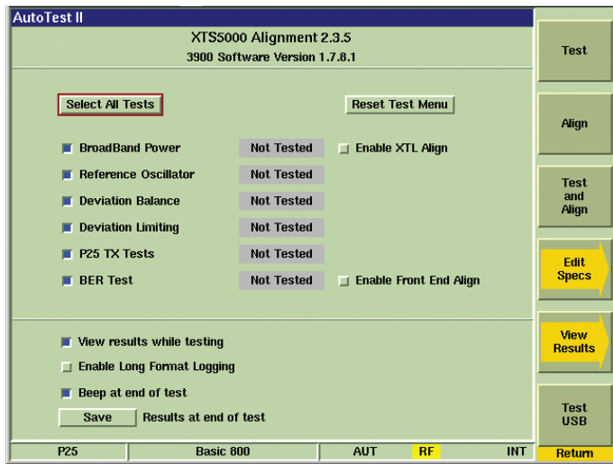
Figure 21. Example of Auto-Test Display
